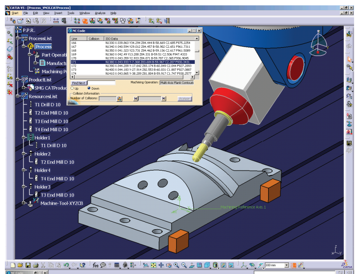
ICAM CE for Machine Verification inside CATIA V5
